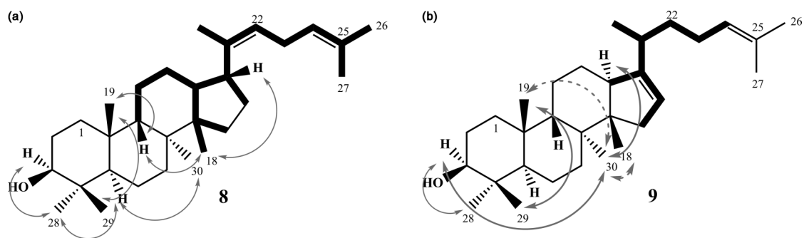
Fig. 1 Bond connectivity and stereochemistry established by HSQC/HMBC (bold bond, \text{—} ) and NOE interaction (curved arrows) of (a) 17 \alpha -protosta-20(22),24-dien-3 \beta -ol ( 8 ) and (b) protosta-16,24-dien-3 \beta -ol ( 9 ).
